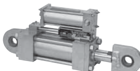
Fig. 200, C-200, 201, C-201 Hydraulic Shock and Sway Suppressor (Snubber) Size Range: Nine standard sizes with load ratings from 3000 (lbs.) to 128,000 (lbs.) Pages 197 - 199
