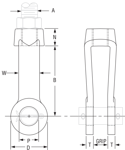
FIG. 299: LOADS (LBS) • WEIGHTS (LBS) • DIMENSIONS (IN)
