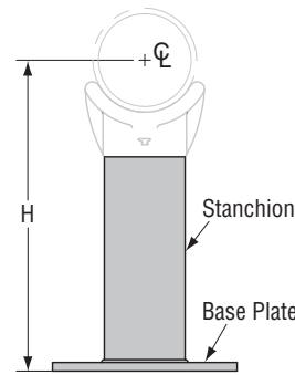
Fig. 63, Type P Square Cut End for use with Figure 258 or 259 Pipe Saddle Support (See pages 109 & 112)
