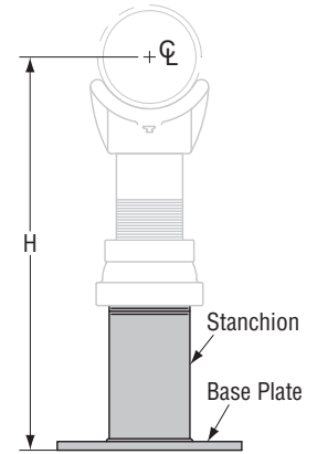
Fig. 63, Type T Square Cut Threaded End for use with Figure 264 or 265 Adjustable Pipe Saddle Support (See pages 110 & 111)
