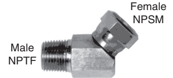
45° Male Pipe x Female Pipe Swivel Nut
