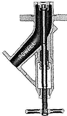
Fig. 2920 Disc opens into tank
