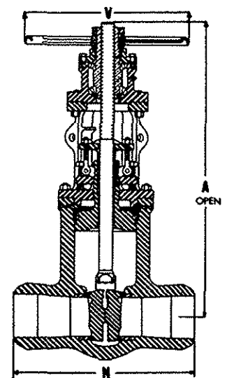
Gate -- Welding Ends Sizes, 4" and 18" 2000 - 2500 Class
