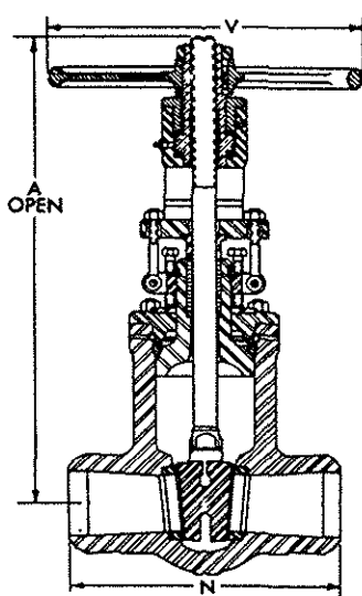
Gate -- Welding Ends Sizes, 2 1/2" - 4" 600 - 1500 Class
