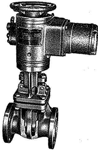
Flanged End. O.S.&Y. Gate Valve with Electric Motor Actuator
