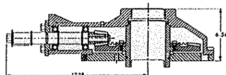
MODEL C-24 ACTUATOR
