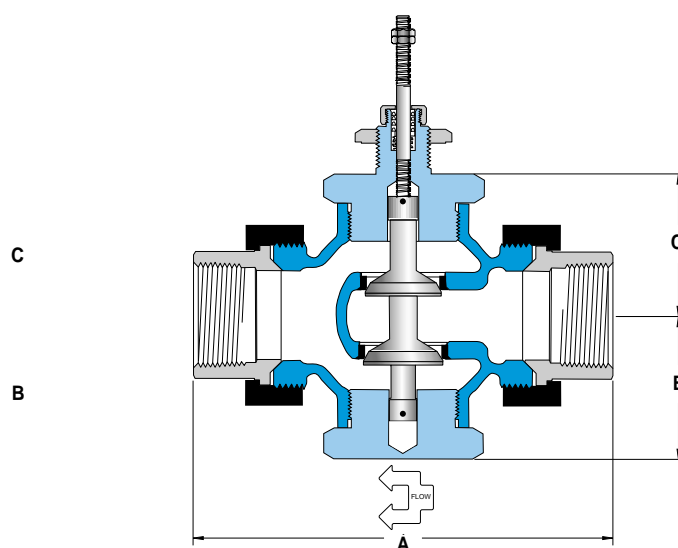
stem In-To-Open
