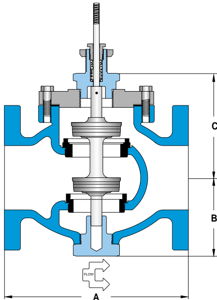
stem In-To-Close
