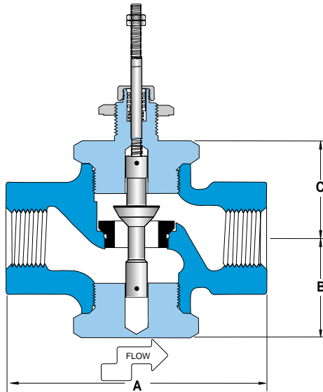
stem In-To-Close
