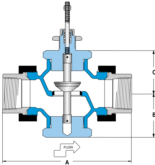
stem In-To-Close
