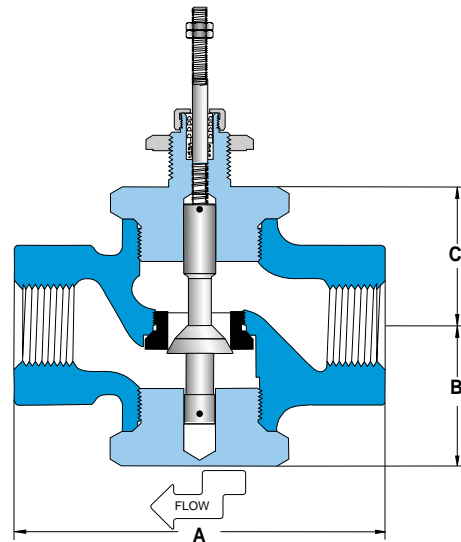
stem In-To-Open
