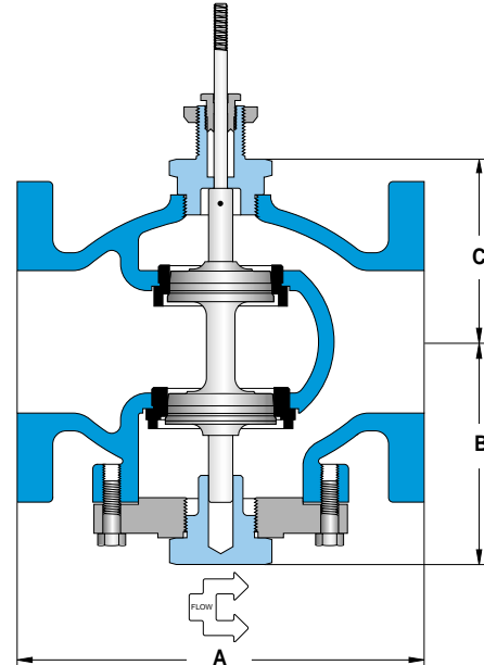
stem In-To-Open
