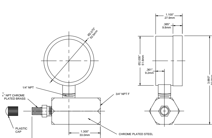
2" Gas Test Gauge
