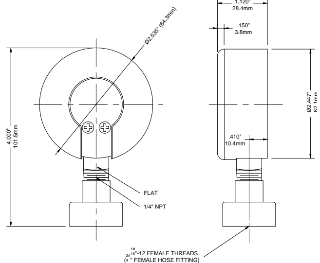
2.5" Water Test Gauge
