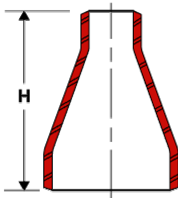
Concentric
